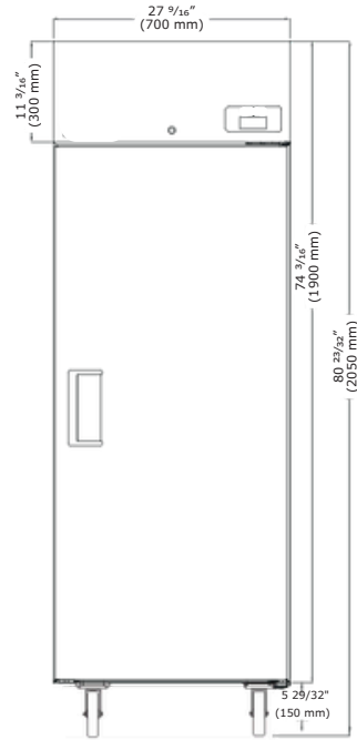
Front (Closed)
