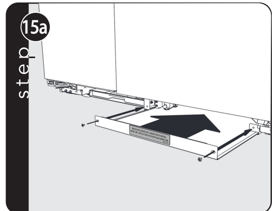
Drive two screws back into place to secure tray in position. If the water line interferes with proper insertion of tray, it may be stored away until unit is to be moved again.
