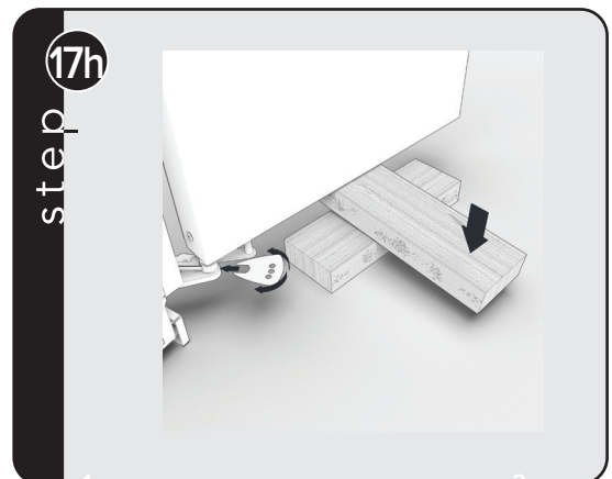
Use a couple of 2x4's to create a fulcrum to take the weight off the door. Insert the spacer adjustment tool into the pivot plate bushing while applying pressure on the fulcrum to remove the door weight, adjust the pivot bushing counterclockwise to raise the door or clockwise to lower the door. Re-assemble the items removed from step 17b thru 17d
