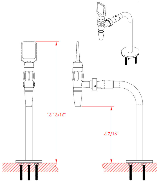
WB-RT-1 Single Round Tower
