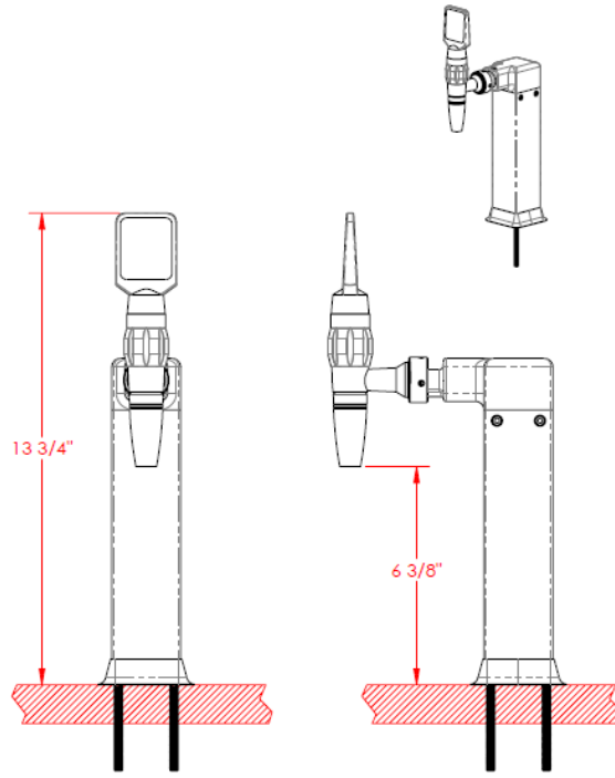
WB-ST-1 Single Square Tower
