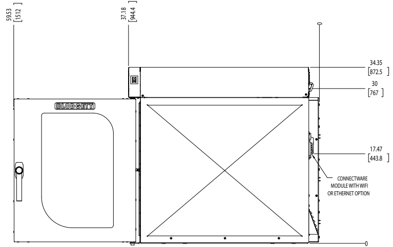
SIDE
