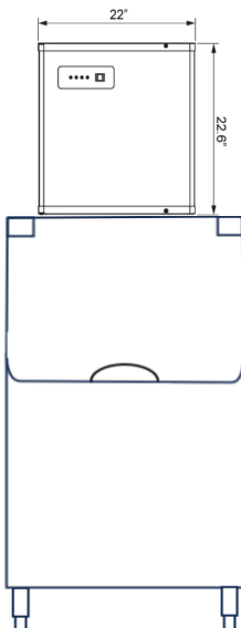
22" unit on 30" bin
