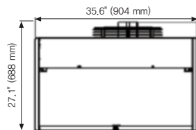
Side-Condenser
