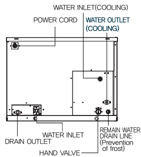
REAR-Water
