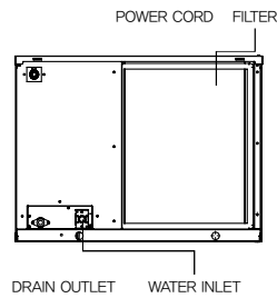
REAR-Air
