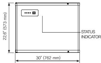
REAR-Water
