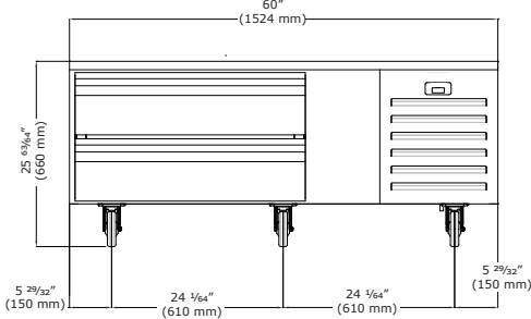
Front (60" Model)
