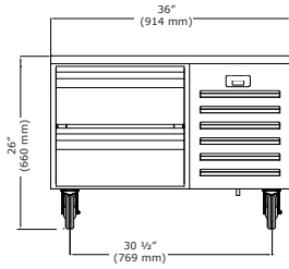
Front (36" Model)
