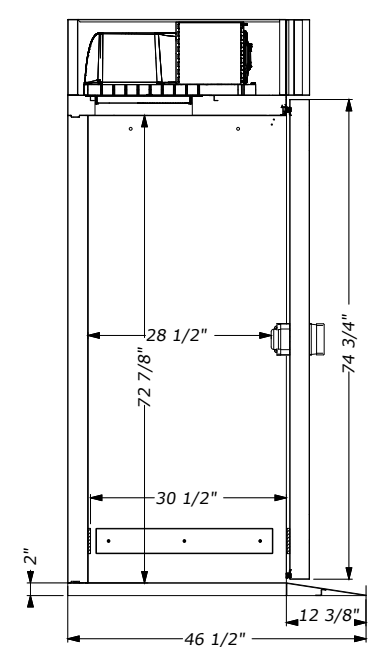
Back UCFZ633/666
