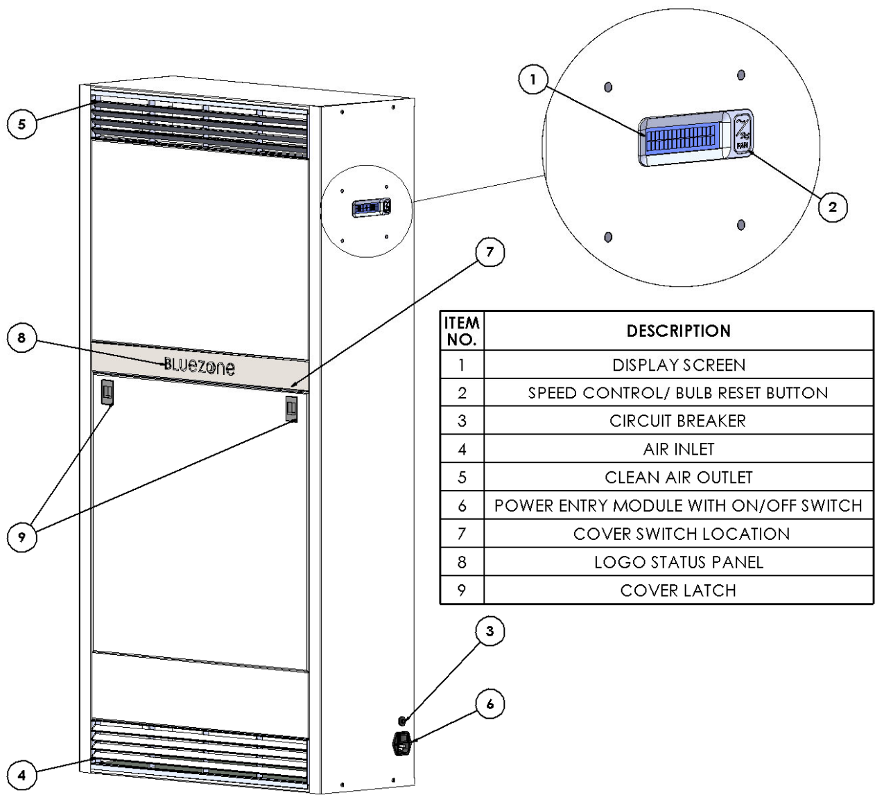
Figure 1: Bluezone PK-220 Key Components
