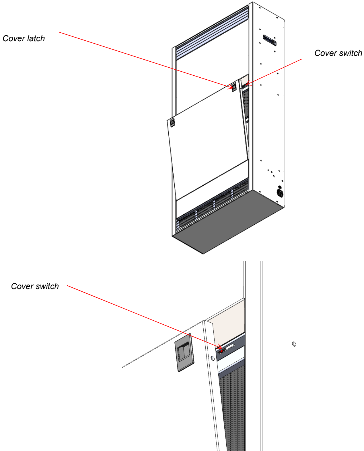
Figure 16: Bluezone PK-220 Cover Switch and Cover Latch
