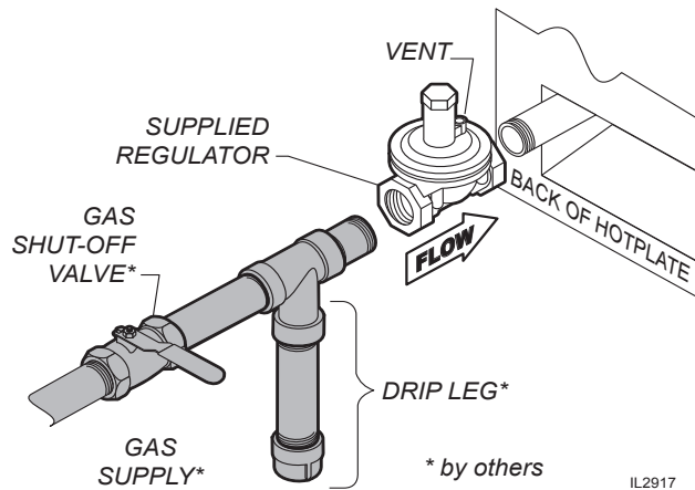
Fig. 2 Gas Supply Piping
