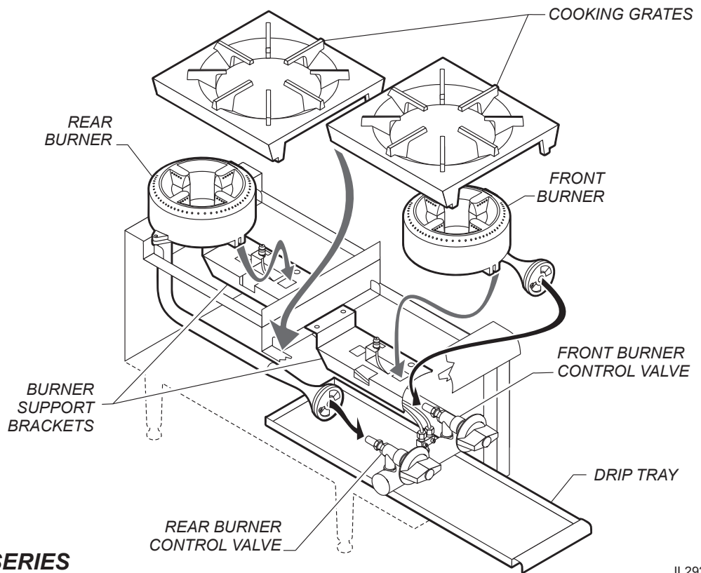
Fig. 5 Hotplate Assembly
