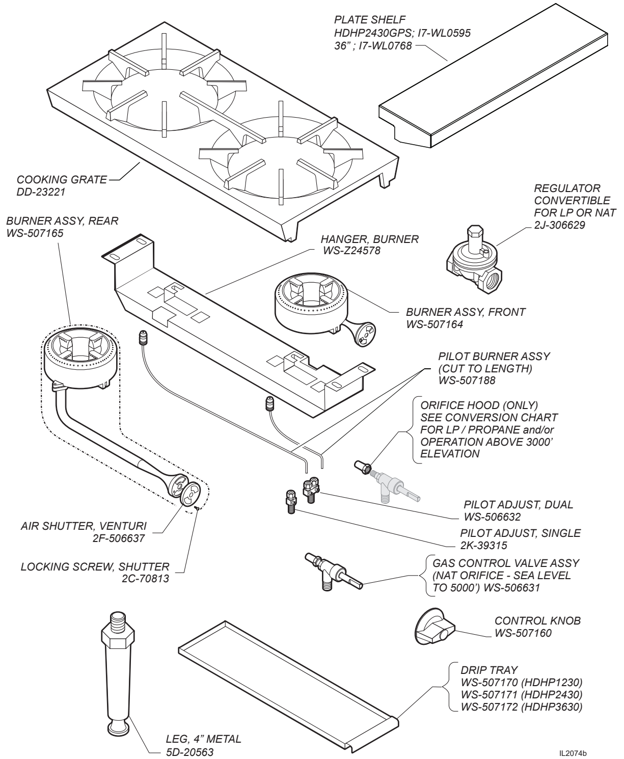
HDHP-SERIES HEAVY DUTY HOTPLATE
